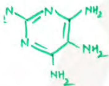
5,6-Tetraminopyrimidine
